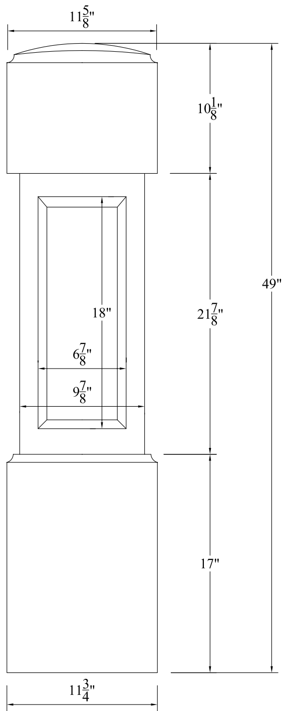
12" RESIDENTIAL POST WITH ROUNDED CAP - EXTENDED/STAIR Not To Scale
